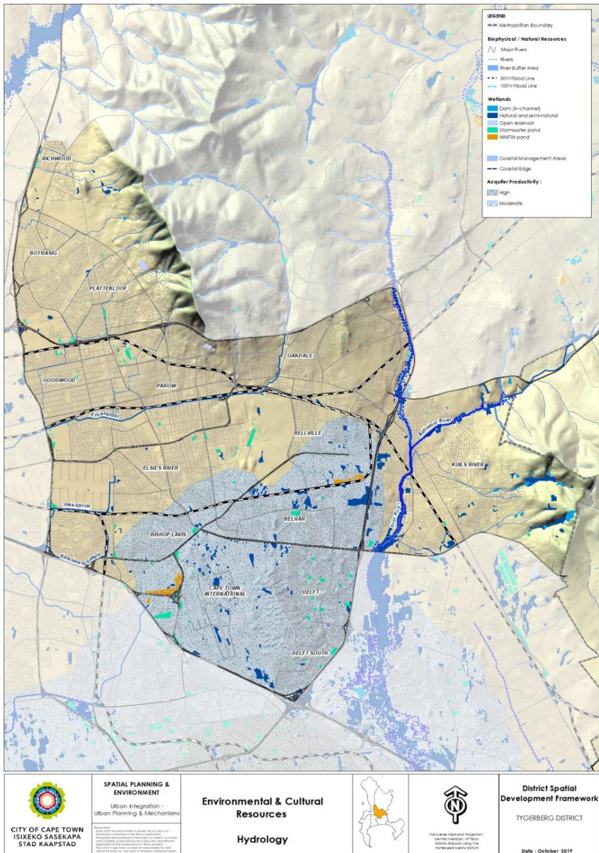
Figure 17: Hydrology
