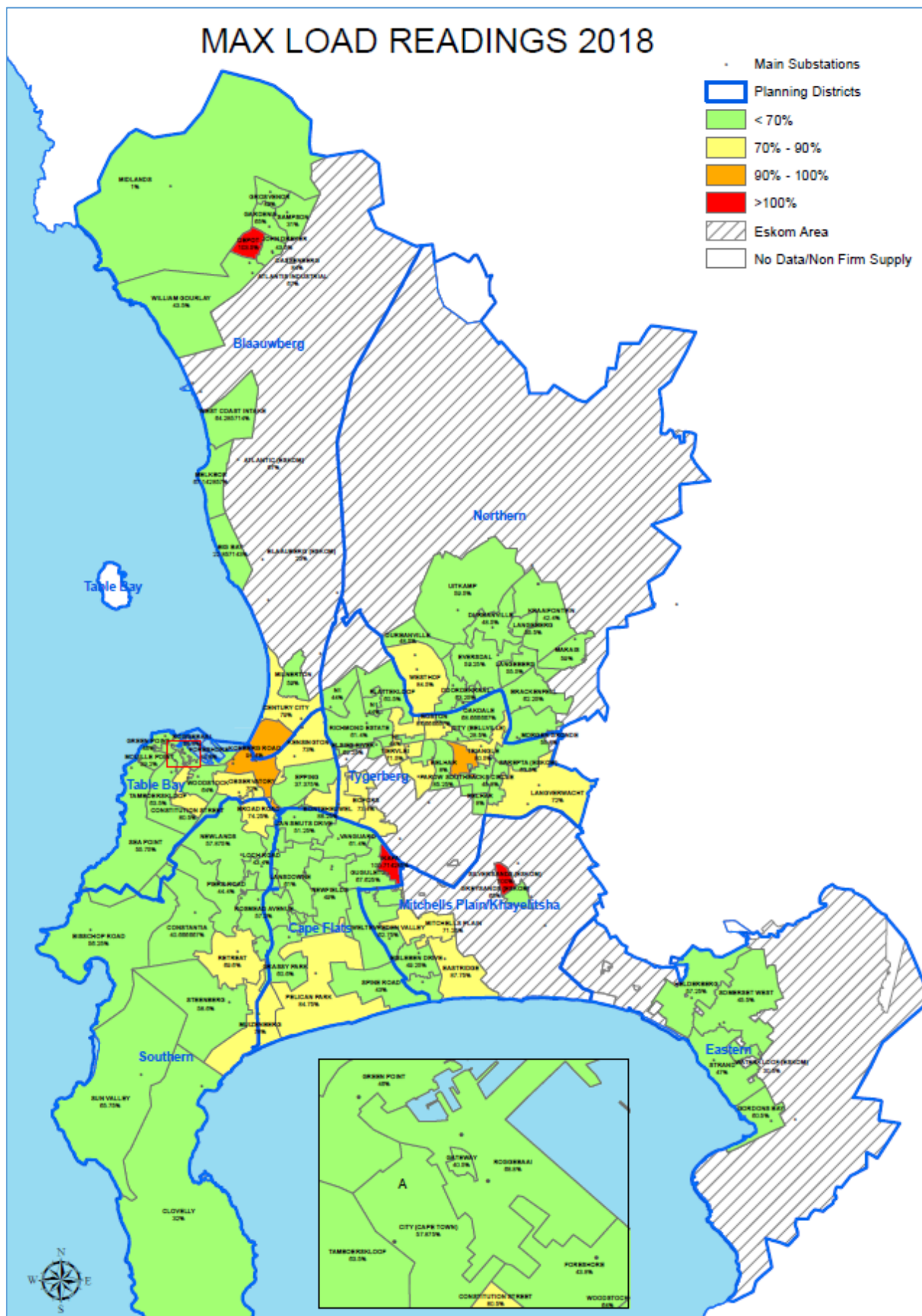
Figure 41: Substation loadings 2018
