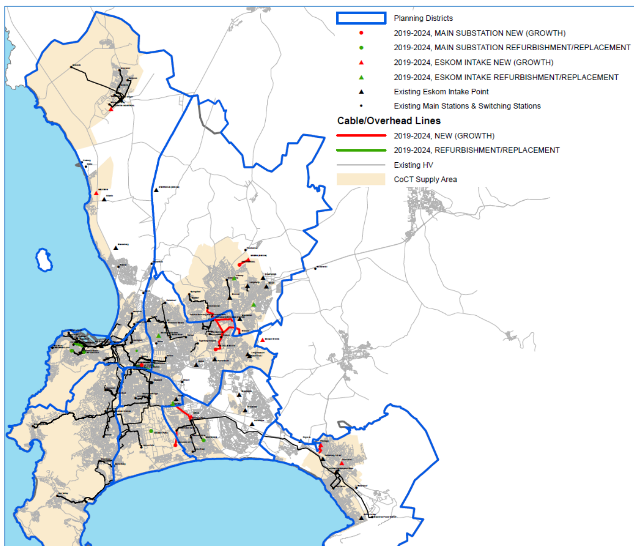
Figure 42: Proposed electricity infrastructure projects
