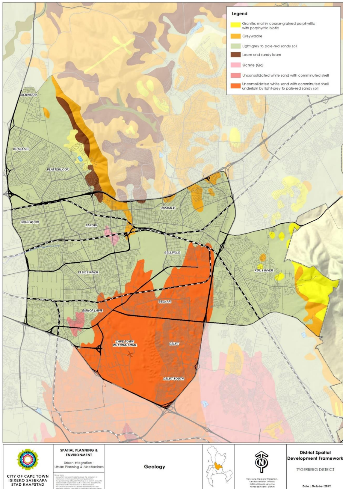
Figure 16: Geology
